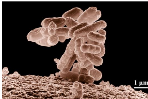
Escherichia coli (E.coli) magnified 10,000 times. E. coli is a simple prokaryotic cell.
