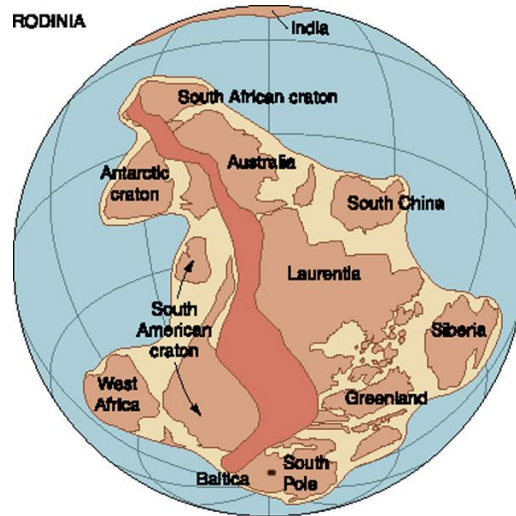
Rodinia as it came together about 1.1 billion years ago.
