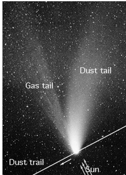
The gases that create a comet
