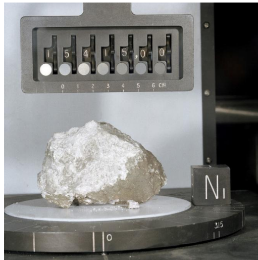
The Genesis Rock was brought back to Earth by the Apollo 15 astronauts.
